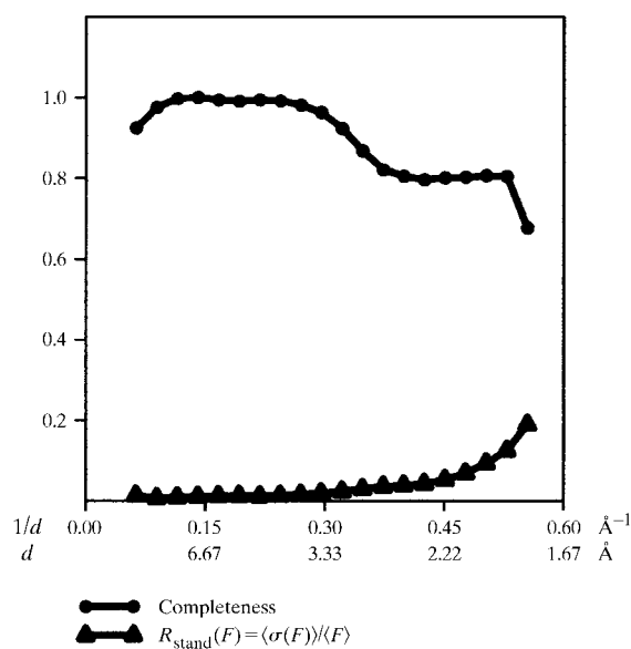
Figure 1 Completeness of data and R_{\text{standard}} of data plotted versus resolution. The figure was prepared using SFCHECK (Vaguine et al. , 1999).
